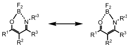
Scheme 3. Possible resonance forms for difluoroboron \beta -ketoiminates.
