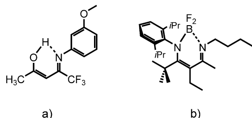
Figure 2. Hypothetical (a) free ligand \text{H}(\text{CH}_3, \text{H}, \text{CF}_3, m\text{-(OMe)C}_6\text{H}_4) and (b) difluoroboron complex \text{BF}_2(t\text{Bu}^{\text{Dipp}}, \text{Et}, \text{Me}^{n\text{Bu}}) Dipp = diisopropylphenyl.
