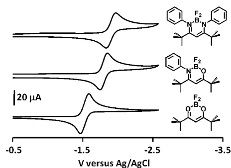
Figure 7. Cyclic voltammograms for \text{CH}_3\text{CN} solutions of \text{BF}_2(\text{tBu}^{\text{Ph}}, \text{H}, \text{tBu}^{\text{Ph}}) (top), \text{BF}_2(\text{tBu}, \text{H}, \text{tBu}^{\text{Ph}}) (middle), and of \text{BF}_2(\text{tBu}, \text{H}, \text{tBu}) (bottom) obtained at a scan rate of 100 mV/s with (\text{NBu}_4)(\text{PF}_6) as supporting electrolyte.
