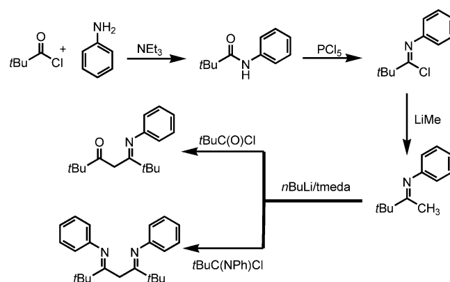
Scheme 2. Preparative route to \beta -ketoimino and \beta -diimine derivatives \text{H}(t\text{Bu}, \text{H}, t\text{Bu}^{\text{Ph}}) and \text{H}(t\text{Bu}^{\text{Ph}}, \text{H}, t\text{Bu}^{\text{Ph}}) .
